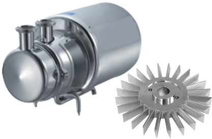
Self-Priming Pumps CIP Return Pumps Liquid Ring Pumps
