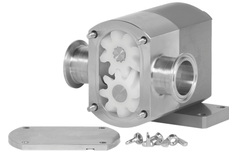
Gear Pumps
