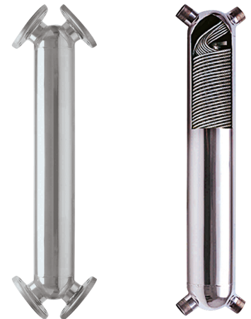
AIC JAD® Heat Exchangers Excellent for Steam, Oil, Hot Water, Thermal Fluid
