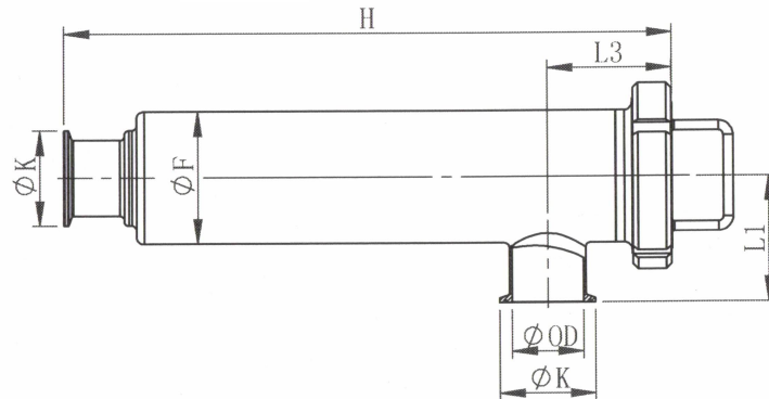
Clamped Angle Type Strainer
