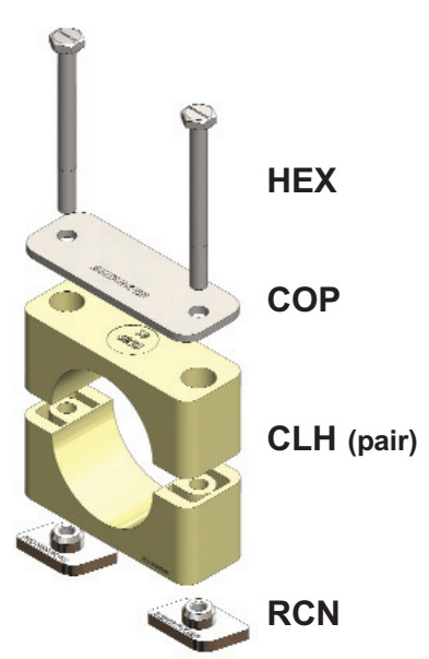
Rail Mount
