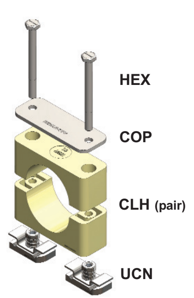
Figure 211 Unistrut Mount
