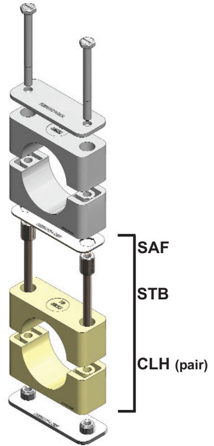
Figure 204 Stacking Kit
