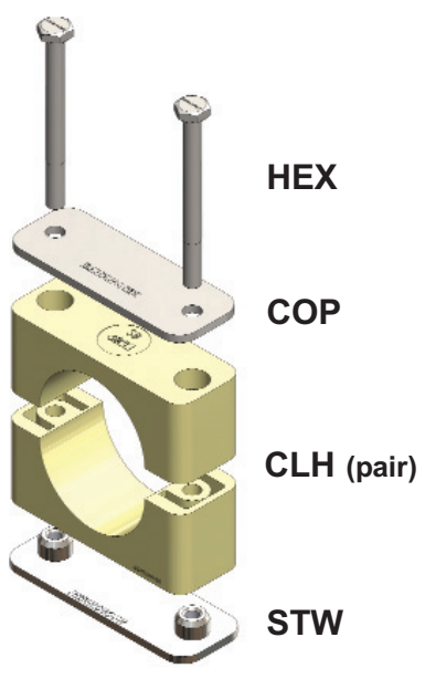
Figure 200 Weld Plate Mount
