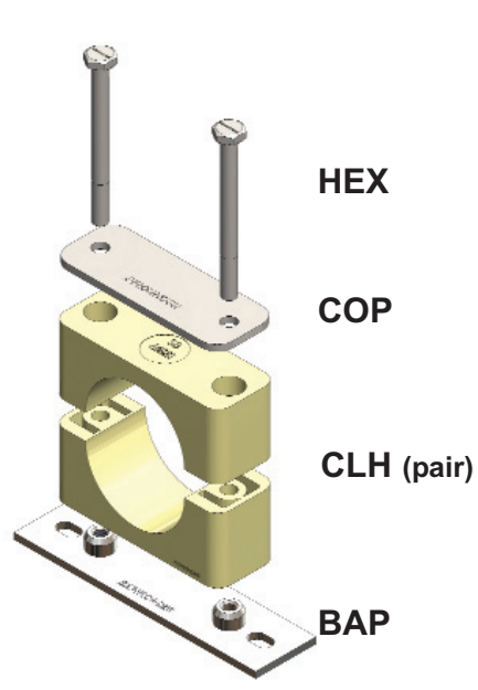
Figure 202 Base Plate Mount
