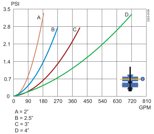
Figure 2. Pressure drop/capacity diagram, upper body
