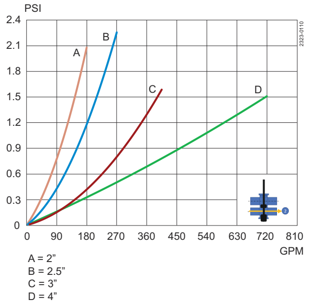
Figure 4. Pressure drop/capacity diagram, lower body
