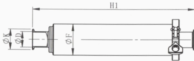
Clamped Straight Strainer
